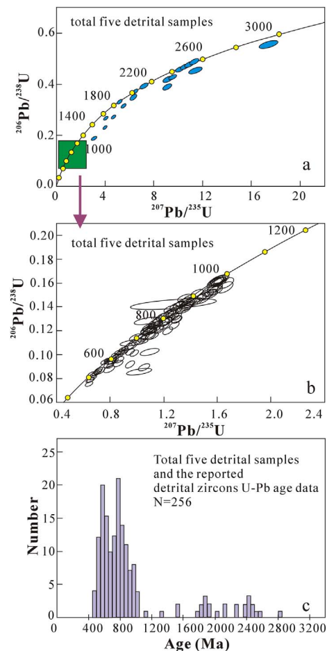
Fig. 8. Concordia and the histogram of ^{206}\text{Pb}/^{238}\text{U} ages of the detrital zircons of the paragneiss samples from the Bulunkuole Group. The data of the age histogram include the five samples analyzed in this study and the data from Zhang et al. (2003), Z.M. Zhang et al. (2012), C.L. Zhang et al. (2012), Yang et al. (2012) and Zheng et al. (2016) (see details in the text).
