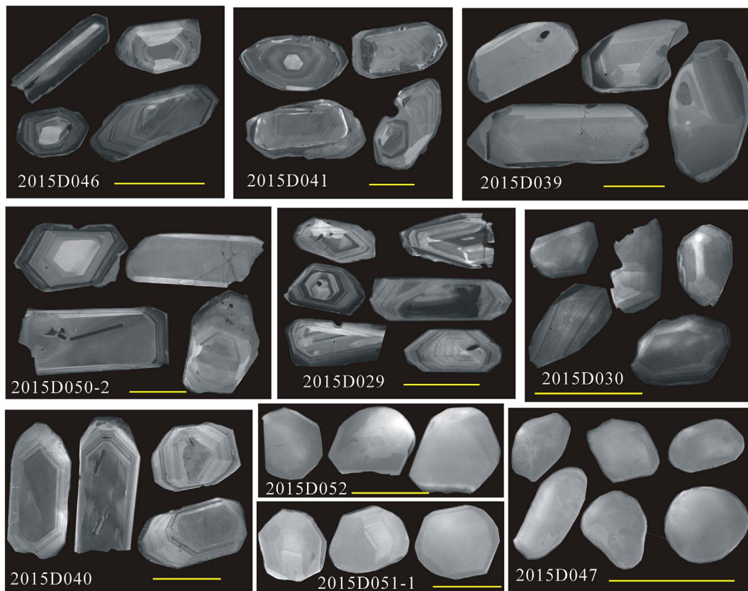
Fig. 9. Representative cathodoluminescence images of the magmatic zircons and metamorphic zircons from the representative igneous rocks, paragneiss, amphibolite (meta-basalt or dolerite) and high-pressure mafic granulite (see details in the text). The scale bar is 100 \mu\text{m} .
