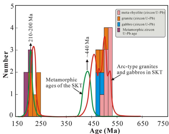
Fig. 13. Histogram of the zircon U-Pb ages of the meta-rhyolite, intrusive rocks and the metamorphic ages of the paragneiss, amphibolite (meta-basalt) and high-pressure mafic granulite.
