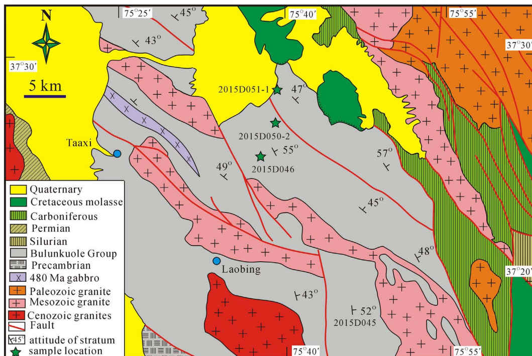
Fig. 3. Geological map of the southern section of the Bulunkuole Group (the Zankan-Laobing iron deposits area).
