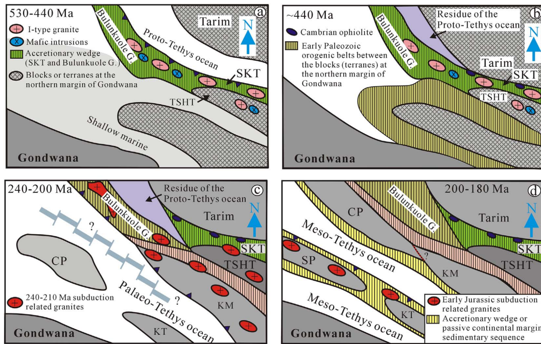
Fig. 14. A schematic diagram to illustrate the tectonic evolution of the NE Pamir Plateau. a - southward subduction of the Proto-Tethys Ocean induced the formation of the Cambrian-Ordovician accretionary wedge (SKT and the Bulunkuole Group); b - at ca. 440 Ma, final assemblage of the blocks (or terranes, including Tarim, Qaidam, Yangtze, South Qiangtang, etc.) to the Gondwana Land; c - northward subduction of the Paleo-Tethys Ocean along the southern margin of the NE Pamir and the TSHT likely began at ca. 240 Ma. During this process, voluminous granites were emplaced along the Kongur Shan mountain in the NE Pamir, the TSHT and the southern belt of the SKT, suggesting that northward subduction continued till to ~200 Ma; d - the closure process of the Palaeo-Tethys Ocean propagated from east to west with final closure at ca. 180 Ma (see details in the text). Abbreviations: CP-central Pamir, SP-south Pamir, QT-Qiangtang terrane, SKT-south Kunlun terrane, TSHT-Tianshuihai terrane, KM-Karakul-Mazar terrane, KT-Karakorum terrane.
